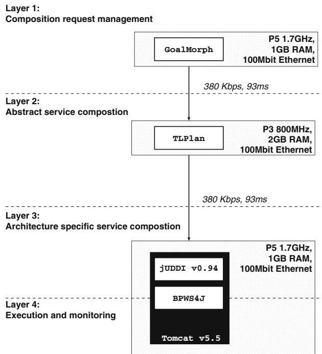
Fig. 9 Experimental setup
