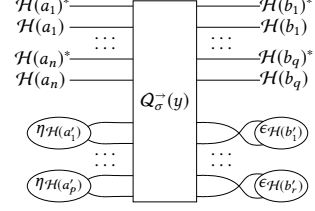
Fig. 13. Reduction \Downarrow_x(Q_\sigma^-(y))
