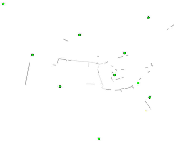
(b) Savitzky-Golay (314)
