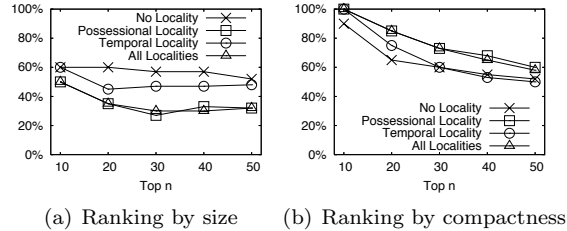
Figure 3. Precision of HAM with respect to the length of ranking for subject Eclipse
