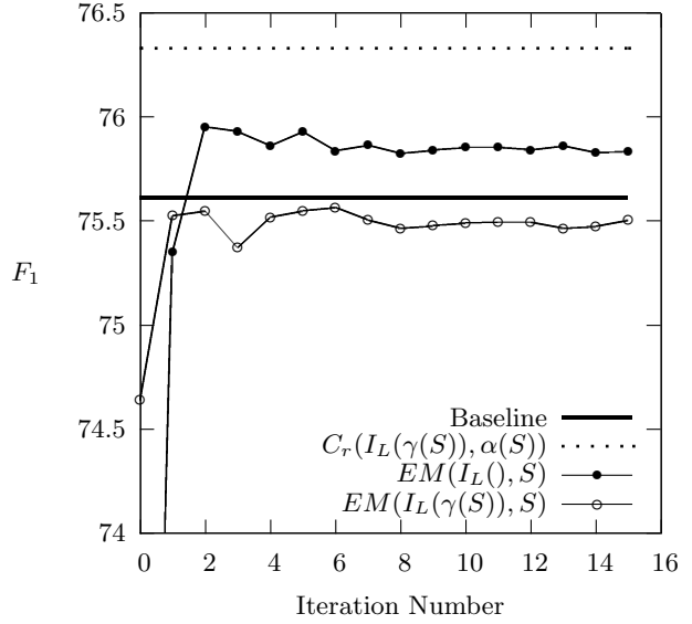
Figure 2: Performance over S for C_r and EM.
