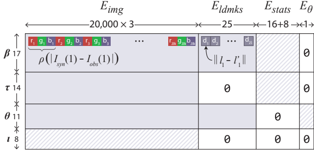
Figure 8: The non-zero structure of our Jacobian J_r for a 200 \times 100 px eye region. J_r is calculated entirely on the GPU. Dashed regions represent sparse blocks.
