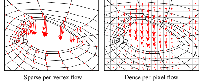
Figure 9: We efficiently convert sparse per-vertex image-space flows (left) to a dense per-pixel flow field (right) using GPU rasterization. We use this dense flow-field to warp the eyelids.
