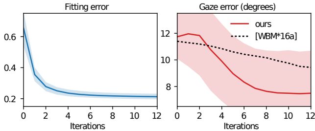
Figure 11: Fitting error and gaze error for the Columbia dataset [SYFN13]. Line is median, filled region is interquartile range. Our second-order optimization strategy converges much faster than previous first-order methods [WBM*16a].
