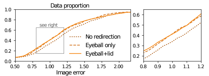
Figure 13: Redirection error decreases as we enable more parts of our redirection pipeline. The x-axis represents image error, and the y-axis represents the proportion of data under that error.
