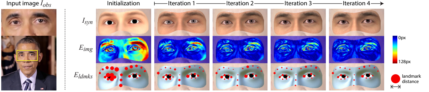
Figure 7: We fit our 3D eye region model to an image by minimizing a reconstruction energy E(\Phi) . Our two main energy terms are a dense photometric error term E_{img} and a sparse landmark similarity term E_{ldmks} . This figure shows the energies decreasing over four iterations of the Gauss-Newton algorithm.
