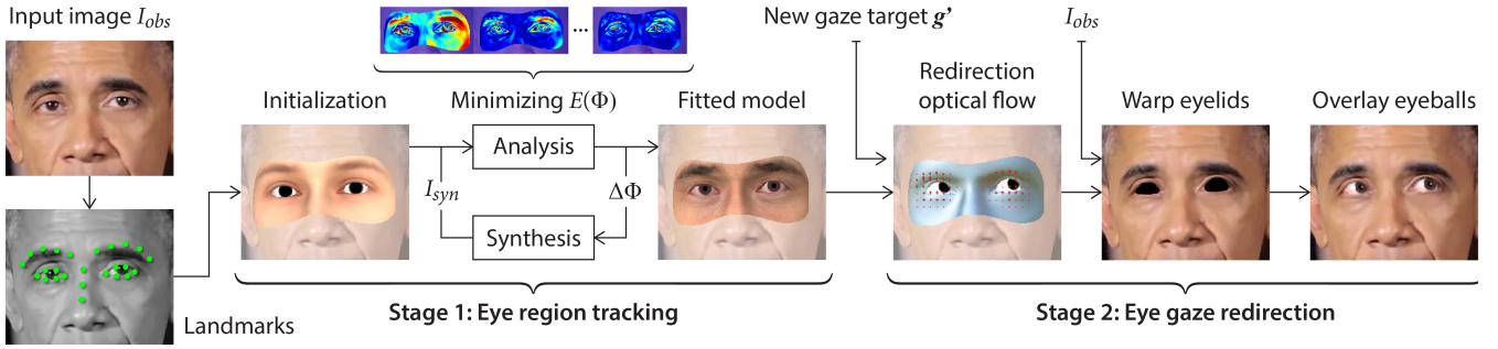
Figure 3: Given observed image I_{obs} , we first initialize our model using 25 facial landmarks from a face tracker [BRM16]. We then find optimal model parameters \Phi^* using analysis-by-synthesis, minimizing a reconstruction energy E(\Phi) . We then modify \Phi^* with the desired gaze and eyelid behaviour, resulting in a new I_{syn} which we blend onto I_{obs} , giving a redirected gaze image.
