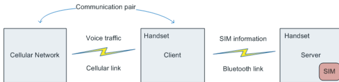
Figure 2: Phone and service monitor (PM).
