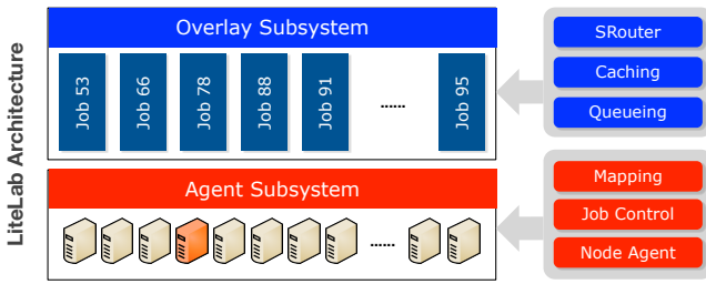
Fig. 1: LiteLab Architecture
