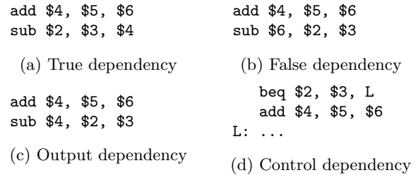
Figure 1: Examples of the different types of dependencies. Examples here are written in MIPS assembly code, where the first operand is the destination register, and the rest are source registers.
