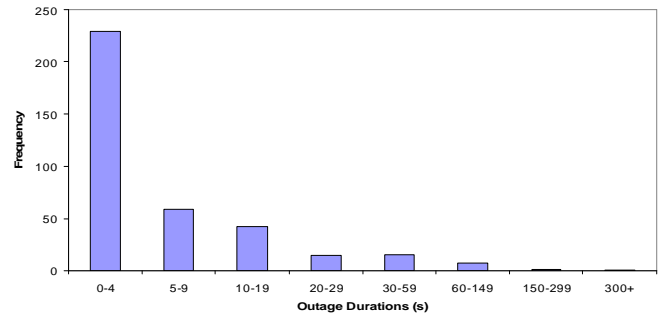
Figure 9: Typical Distribution of Outage Durations with 700 nodes
