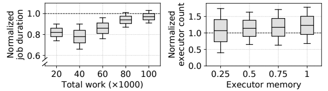
Figure 12: Decima outperforms Graphene* with multi-dimensional resources by (a) completing small jobs faster and (b) use “oversized” executors for small jobs (smallest 20% in total work).
