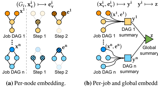
Figure 5: A graph neural network transforms the raw information on each DAG node into a vector representation. This example shows two steps of local message passing and two levels of summarizations.
