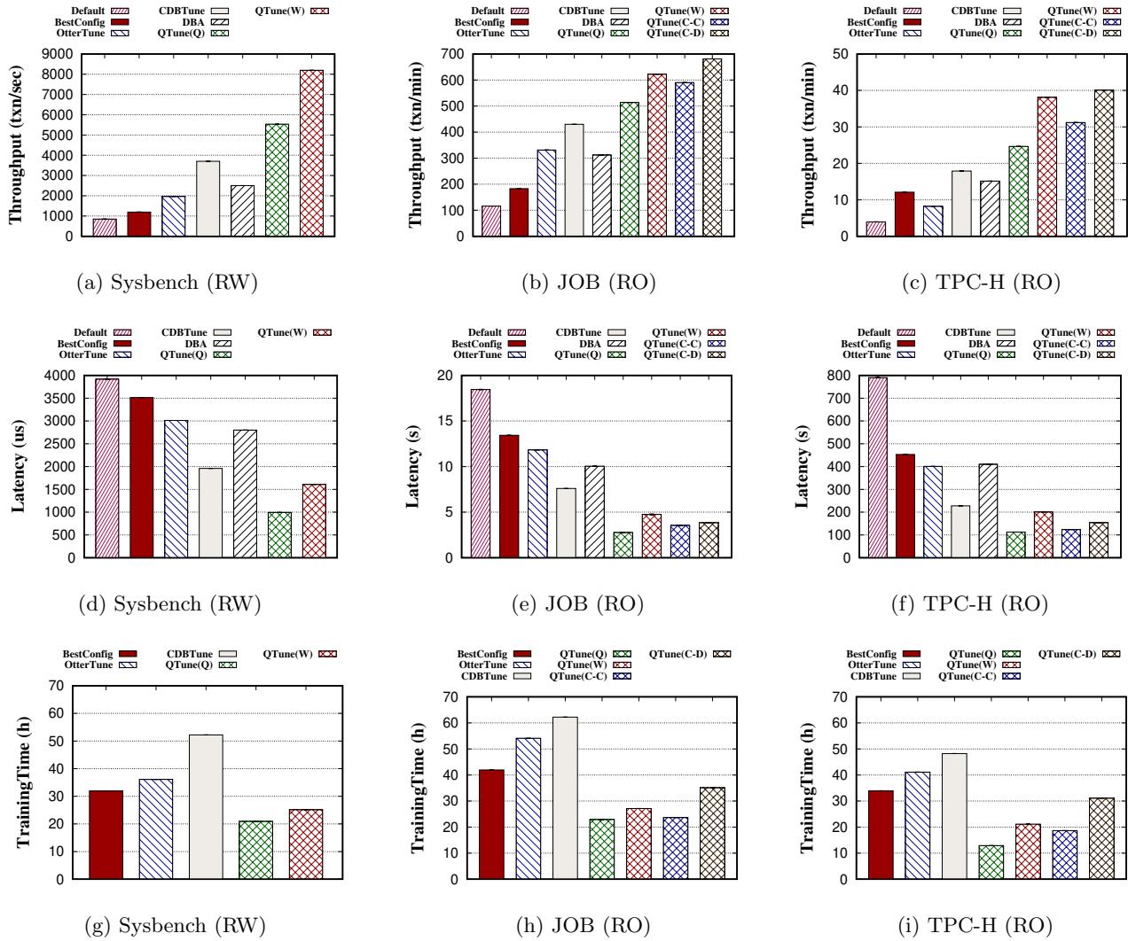
Figure 8: Comparison with existing methods Default settings, BestConfig, OtterTune, CDBTune, DBA on Sysbench (RW), JOB (RO) and TPC-H (RO) on PostgreSQL. Q Tune (Q) represents query-level tuning. Q Tune (W) represents workload-level tuning. And Q Tune (C-C) and Q Tune (C-D) indicate cluster-level tuning using Continuous Tuner and Discrete Tuner respectively.
