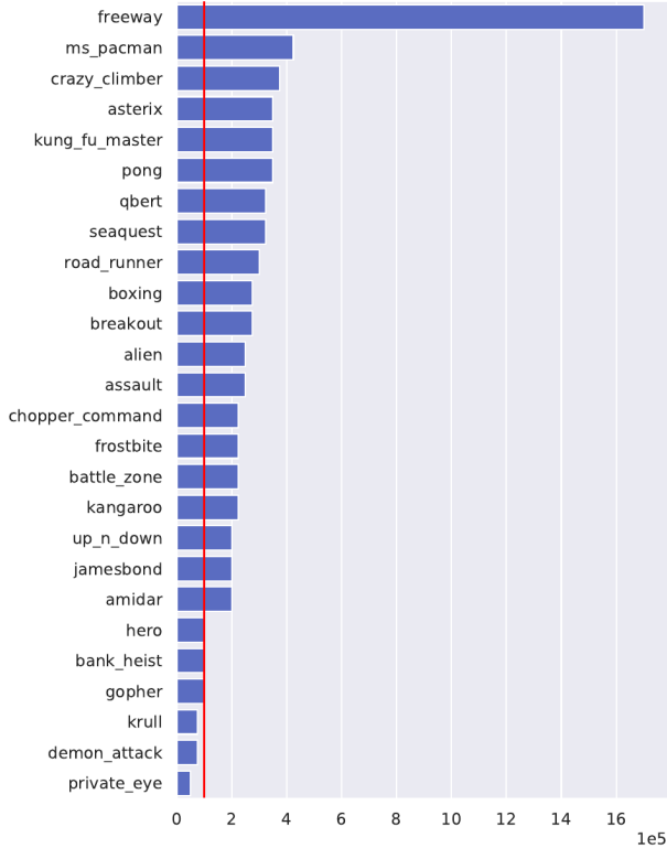
Figure 3. Comparison with Rainbow. Each bar illustrates the number of interactions with environment required by Rainbow to achieve the same score as our method (SimPLe). The red line indicates the 100K interactions threshold used by our method.
