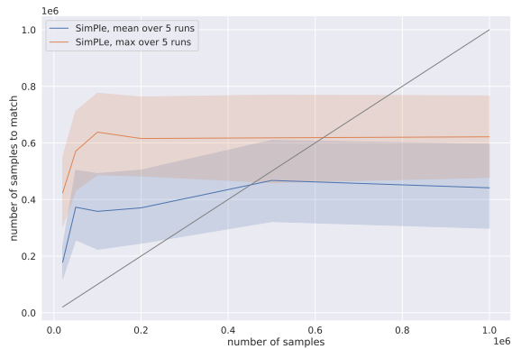
Figure 11. Behaviour with respect to the number of used samples. We report number of frames required by PPO to reach the score of our models. Results are averaged over games.
