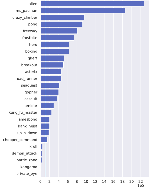
Figure 4. Comparison with PPO. Each bar illustrates the number of interactions with environment required by PPO to achieve the same score as our method (SimPLe). The red line indicates the 100K interactions threshold which is used by our method.
