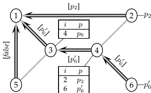
Figure 9: Opportunistic UR Processing
