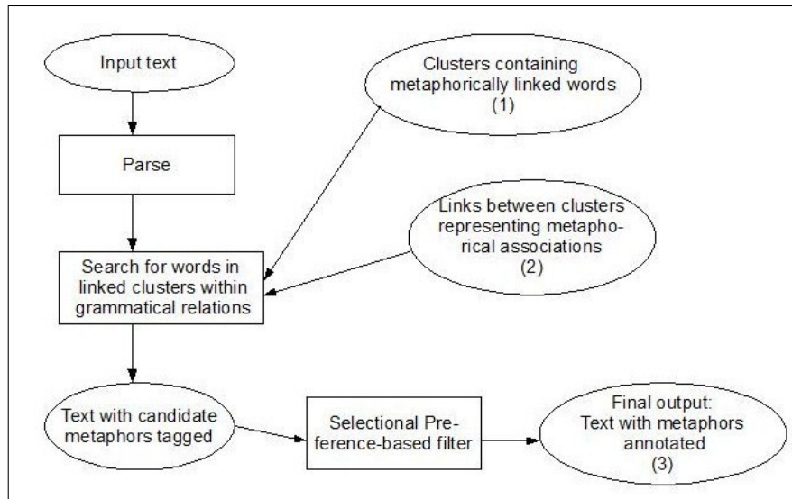
Figure 5 Identification of new metaphorical expressions in text
