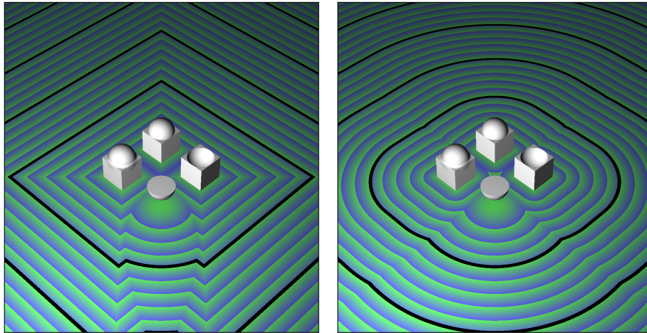
Figure 5: Side-by-side comparison of two implementations of the cube() distance function. On the left, by choosing the absolute maximum distance along each axis, we return unnecessarily far distances along the axes |X|=|Z| . On the right, by choosing length(p) , we achieve a tighter upper bound on the distance function along the |X|=|Z| lines.
