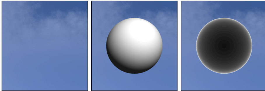
Figure 2: If you have set the tick up correctly, you will see a cloudy blue sky. Use the mouse to spin your point of view (but there's not much to see). If you uncomment the line which calls sphere() in the raymarch() method of fragment_shader.glsl , a sphere should appear. Press R to visualize the number of raymarching steps per pixel of the sphere (black = min, white = max).
