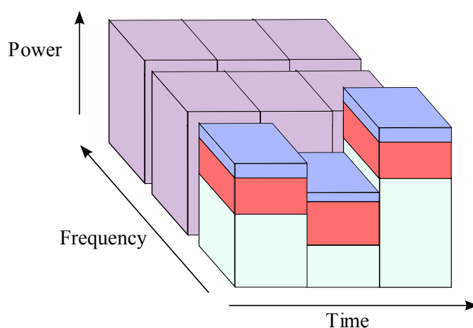
Figure 2.3: How channels are allocated in the time-frequency-code space for W-CDMA. All users from one provider transmit on the same frequency. Each user's power varies over time, as controlled by the base station. Each user has a different spreading code (different colour), giving between 8 and 384 Kbit/s depending on the demands of the traffic [108].
