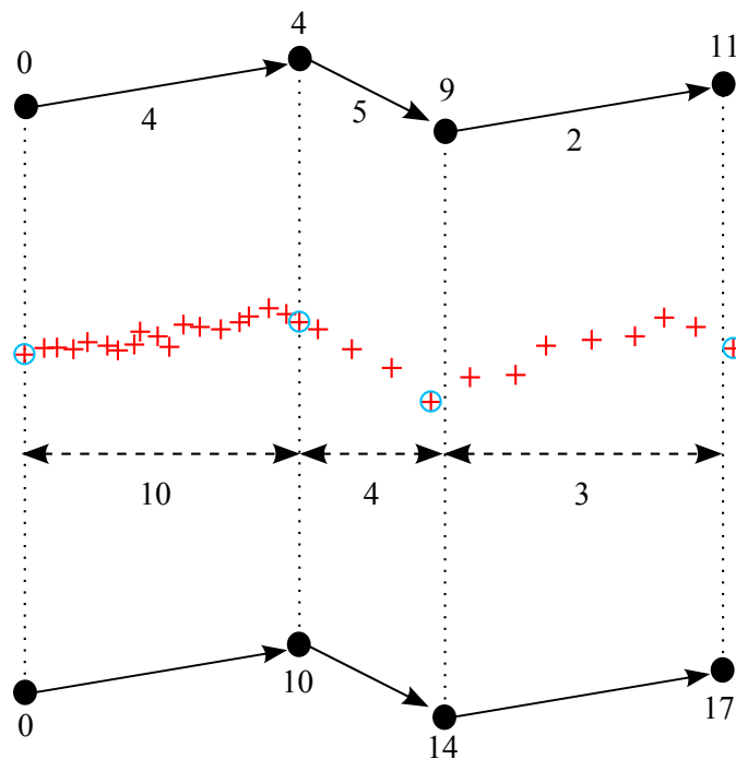
Figure 6.4: Edge traversal times on the proposed route (top) are updated according to the GPS trace (middle). The time taken to travel between each junction is found, and used to update the edge traversal times, giving an corrected route (bottom).
