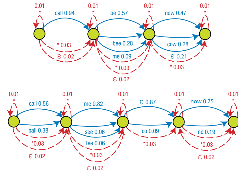
Figure 3. Merging probabilistic text-entry modalities to achieve smarter error correction. In this case, the user intended to type or speak “call me now,” but the system inadvertently output “call be now.” The merge algorithm takes two word-confusion networks as inputs from different text-entry modalities (blue solid lines) and then, using some of the probability mass in each word-confusion cluster, softens the networks by adding epsilon and wildcard transitions (red dashed lines). Epsilon transitions let the algorithm proceed to the next cluster without generating a word. Wildcard transitions indicate that the algorithm can either stay in the same cluster and generate any word (self-loops), or proceed to the next cluster and generate a wildcard word that matches any word. Thereafter, the algorithm searches for the highest joint probability path through both networks using a token-passing model.
