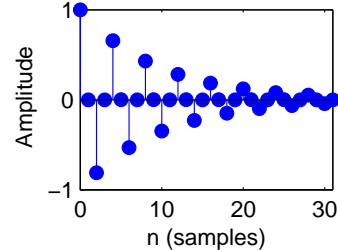
Impulse Response
