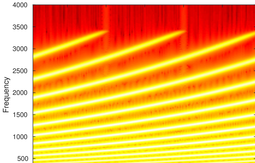
Spectrogram of the first 3 s:
