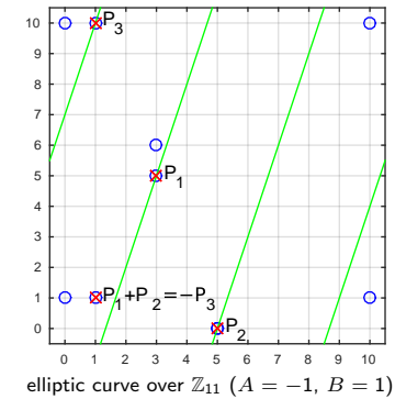
elliptic curve over \mathbb{Z}_{11} ( A = -1, B = 1 )
