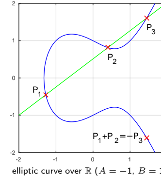
elliptic curve over \mathbb{R} ( A = -1, B = 1 )
