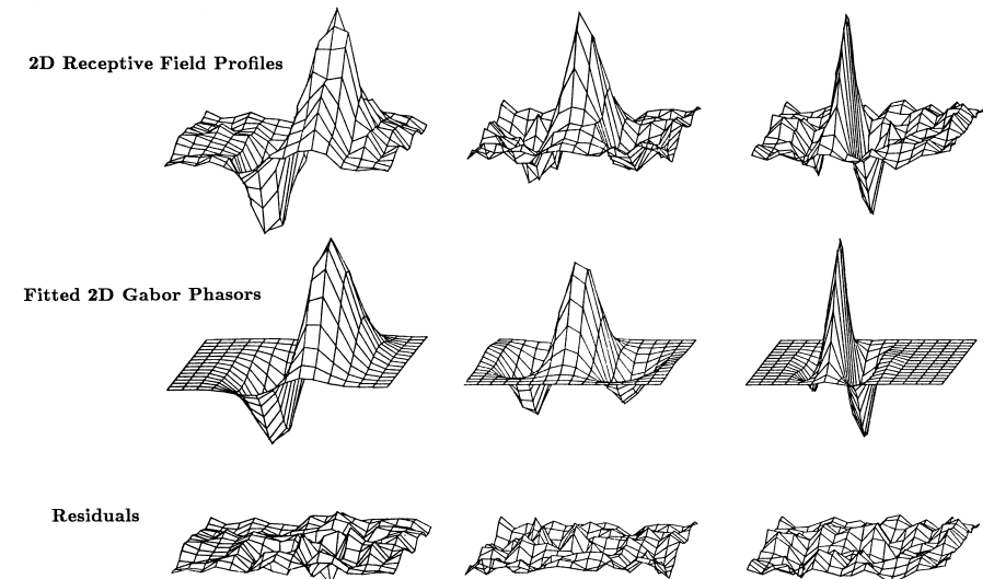
Below: detailed receptive field structure of such neurones (top row); theoretical 2D Gabor phasor components (middle row); and residual differences between the data and models (bottom row).
