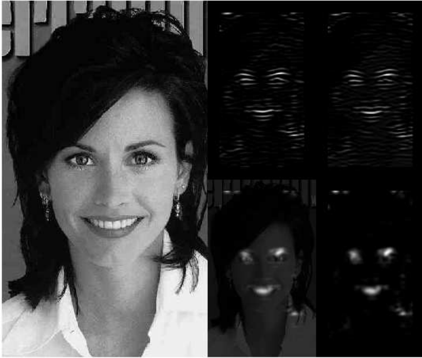
Illustration of Facial Feature Detection by Quadrature Filter Energy. Left panel: original image. Right panel (clockwise from top left): the real part after 2D Gabor wavelet convolution; the imaginary part; the modulus; and modulus superimposed on the original (faint) image, illustrating successful feature localisation by the Quadrature Demodulator Network in the previous Figure.
