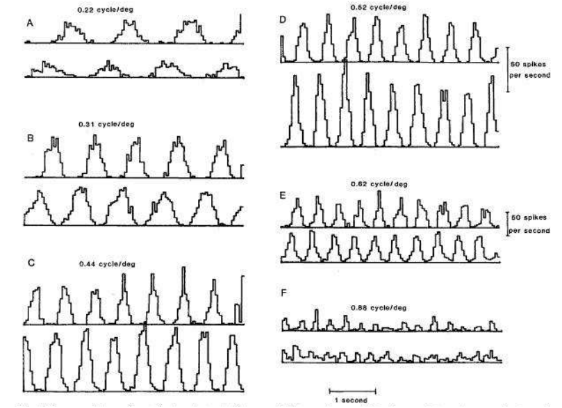
Above: quadrature phase ( 90^\circ ) relationship between adjacent pairs of identically-tuned cortical simple cells, in response to drifting sinusoidal gratings, suggesting complex phasor processing.
