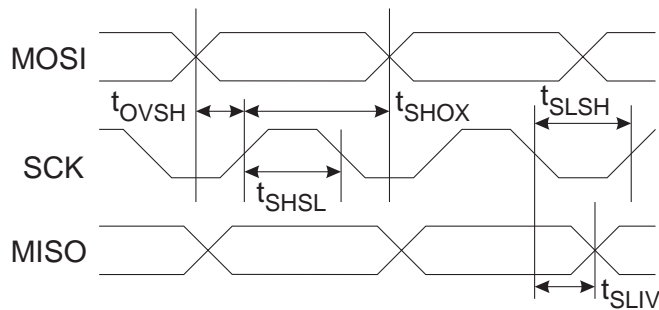
Figure 24-5. Serial Programming Timing
