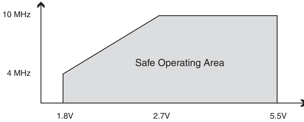
Figure 24-1. Maximum Frequency vs. V_{CC}
