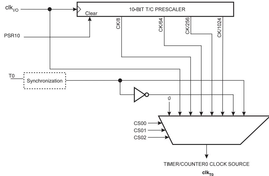
Figure 14-2. Prescaler for Timer/Counter0
