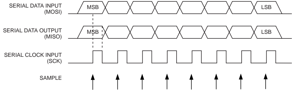
Figure 24-4. Serial Programming Waveforms
