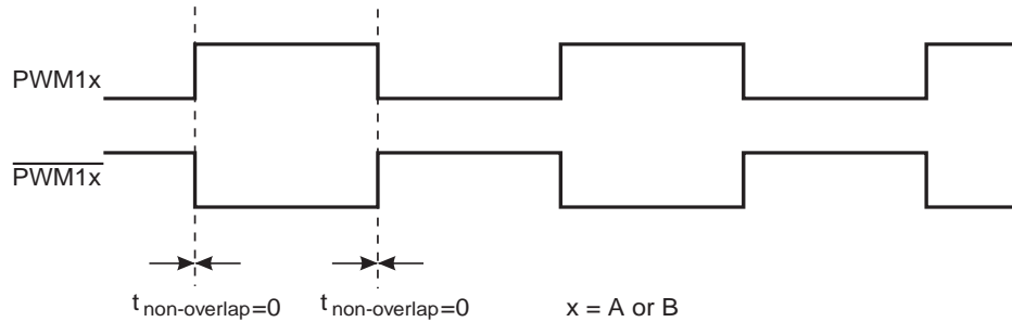
Figure 15-4. The PWM Output Pair
