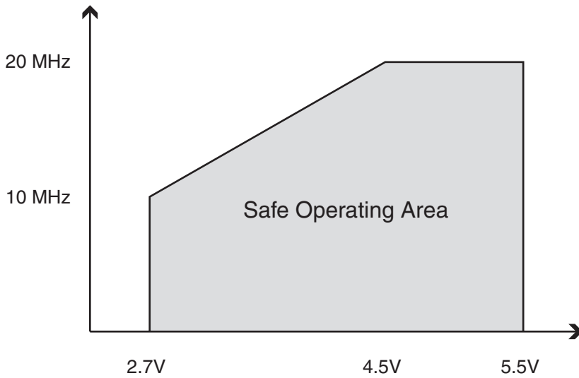
Figure 24-2. Maximum Frequency vs. V_{CC}
