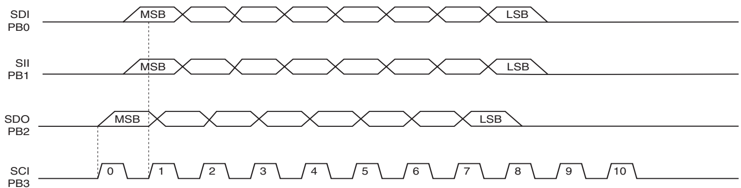
Figure 23-5. High-voltage Serial Programming Waveforms
