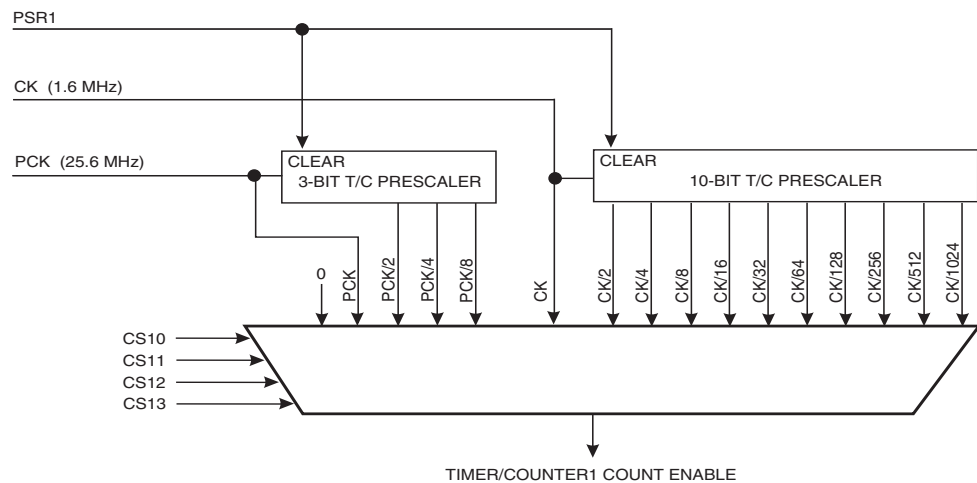
Figure 16-1. Timer/Counter1 Prescaler
