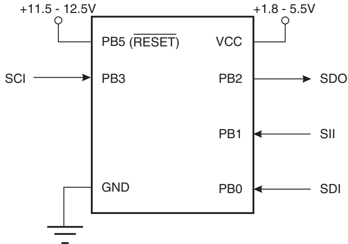
Figure 23-3. High-voltage Serial Programming
