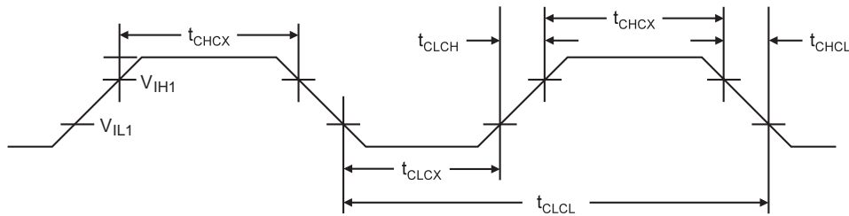
Figure 24-3. External Clock Drive Waveforms
