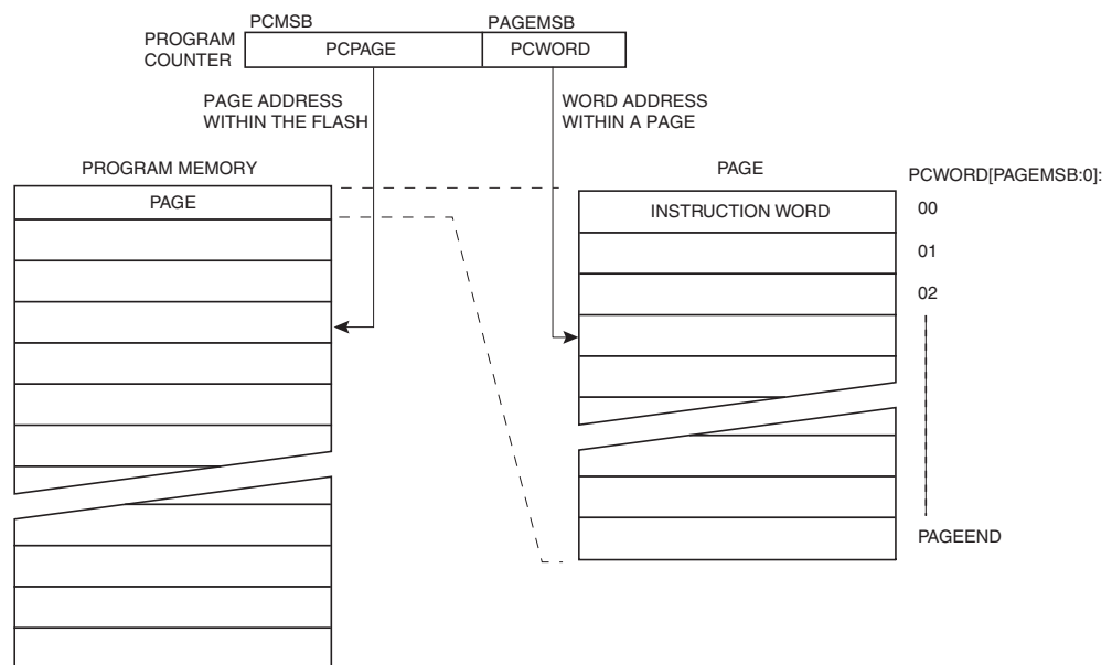
Figure 23-4. Addressing the Flash which is Organized in Pages
