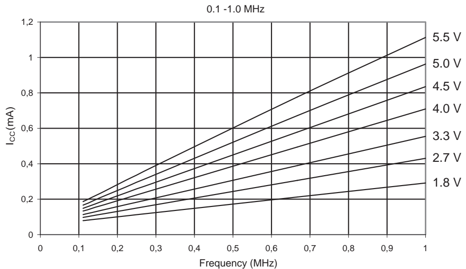
Figure 25-1. Active Supply Current vs. Low frequency (0.1 - 1.0 MHz) ACTIVE SUPPLY CURRENT vs. LOW FREQUENCY
