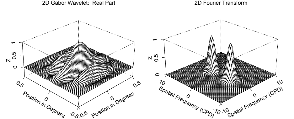
Figure 1: The real part of a 2D Gabor wavelet, and its 2D Fourier transform.
