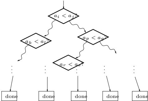
Figure 1: The computation tree for a sorting algorithm
