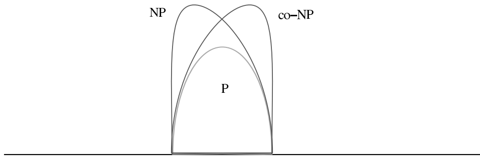
Figure 9: Relation between the classes P , NP and co-NP
