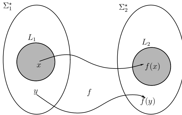
Figure 5: Reduction
