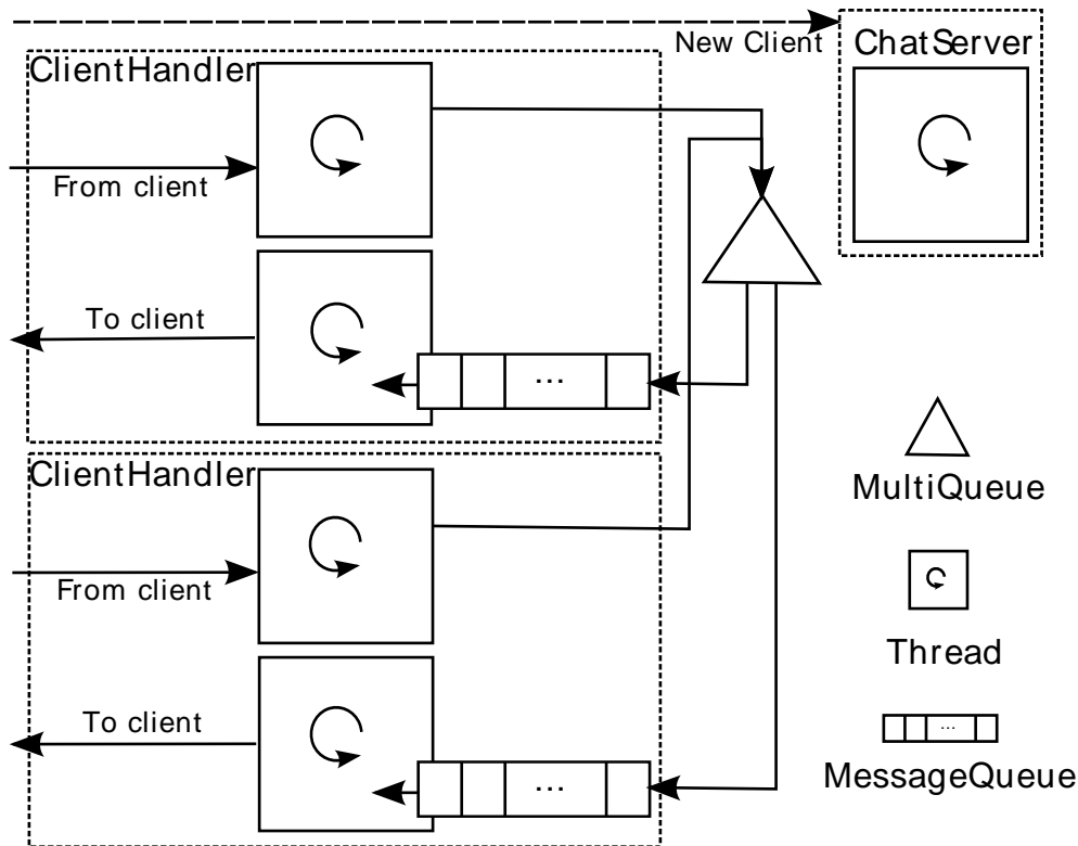
Figure 1. The major Java objects and message flows in the Java chat server
