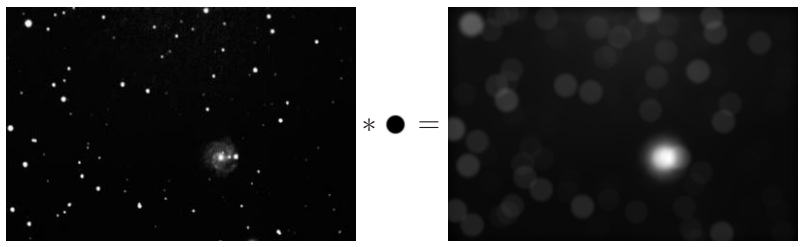
Point-spread function h (disk, r = \frac{as}{2f} ):
