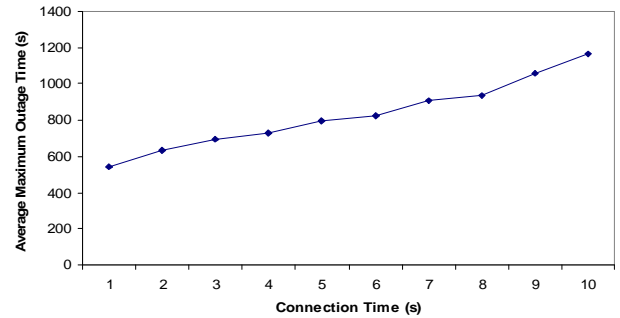
Figure 13: Average Maximum Outage Time vs. Connection Time
