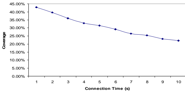
Figure 11: Coverage Variation with Connection Time
