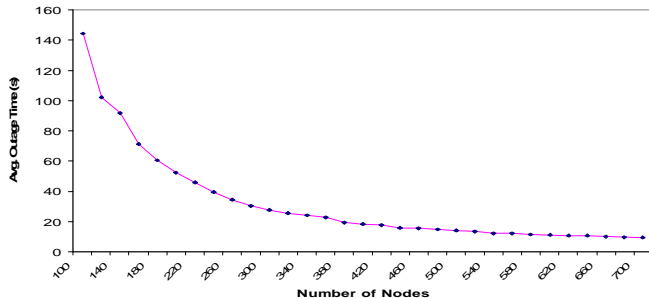
Figure 7: Average Outage Time as Function of No. of Nodes
