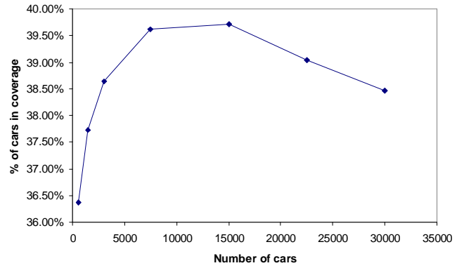
Figure 21: Coverage as Function of Congestion
