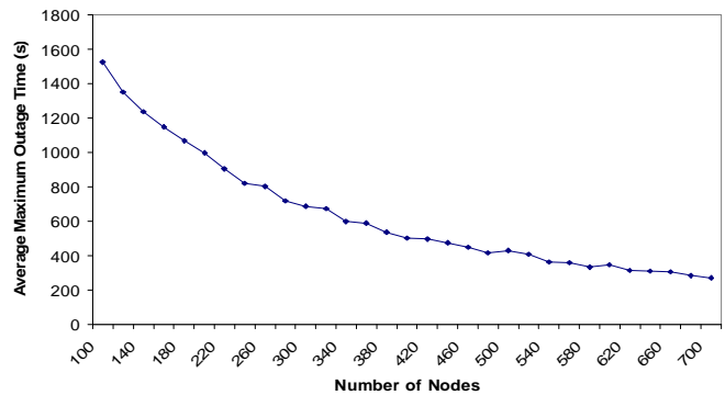
Figure 8: Average Maximum Outage Time as a Function of the No. of Nodes
