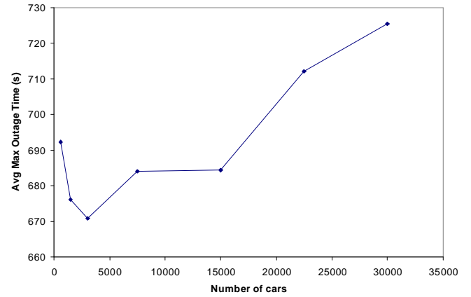
Figure 23: Average Maximum Outage Time
