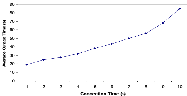
Figure 12: Average Outage Time vs. Connection Time
