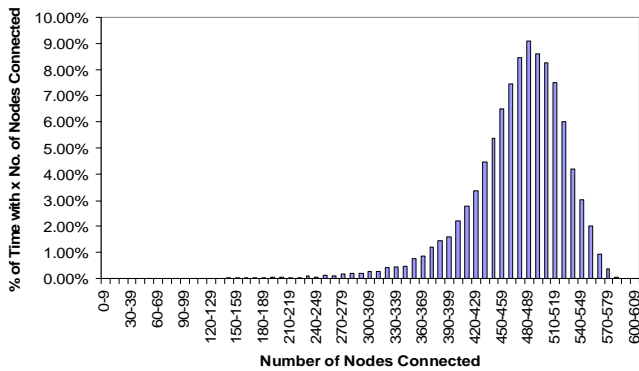
Figure 6: Typical Distribution of Coverage with 700 nodes
