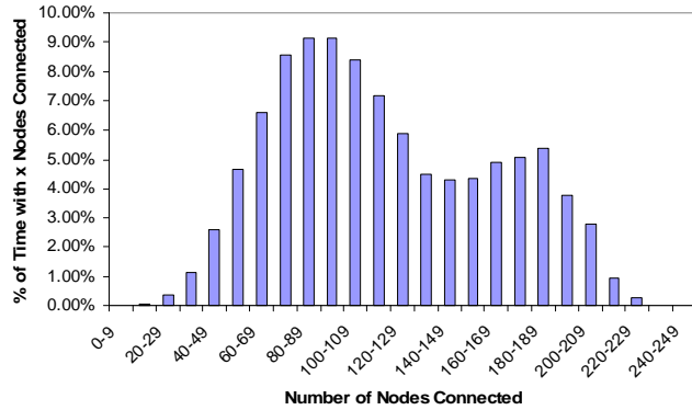
Figure 18: Typical Distribution of Coverage with Congestion (30,000 cars)
