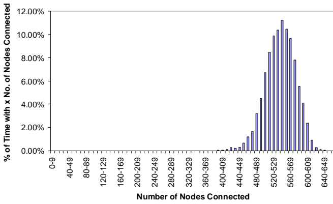
Figure 15: Typical Coverage with 700 Nodes and a 1s Connection Time
