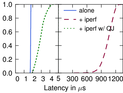
(a) CDF of ping packet latency across a switch. Note the change in x-axis scale.
