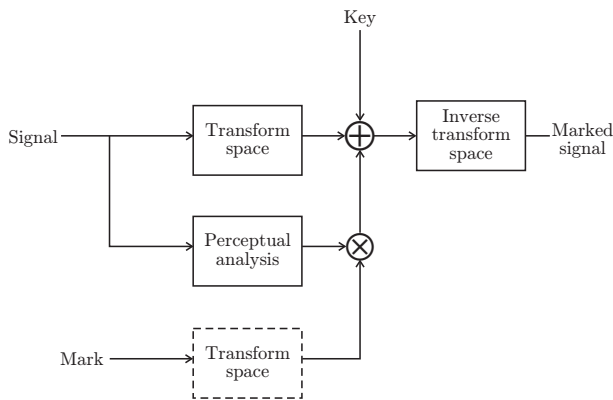
Fig. 5. A typical use of masking and transform space for digital watermarking and fingerprinting. The signal can be an image or an audio signal. The perceptual analysis is based on the properties of the human visual or auditory systems respectively. \oplus corresponds to the embedding algorithm and \otimes to the weighting of the mark by the information provided by the perceptual model.
