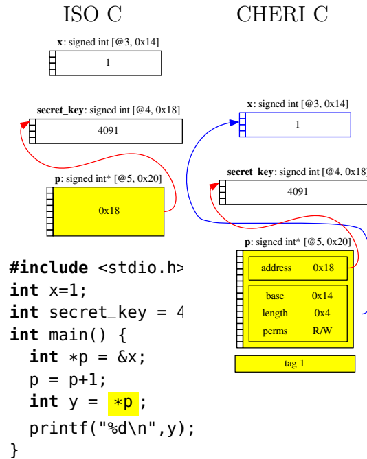
Figure 2: Comparing ISO C with CHERI C. In ISO C the (flawed) program on the left has undefined behaviour, but in practice can leak the secret key. In CHERI C the same program has defined behaviour and will always trap with a hardware exception, because the address used for the *p access is not within the footprint of the capability.
