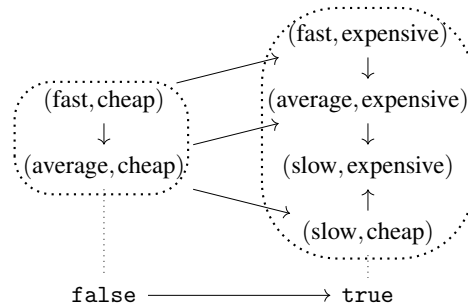
(b) Fibre representation of a boolean profunctor.
