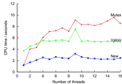
(b) Non-reference-counted algorithms with keys 0...255.
