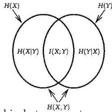
Venn Diagram: Relationship between entropy and mutual information.
