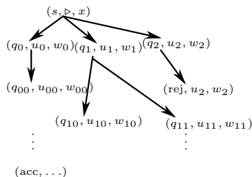
Figure 2: Nondeterministic computation
