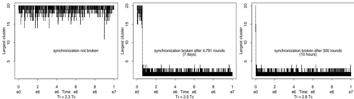
Figure 10: Simulations starting with synchronized updates, for different values for T_r .
