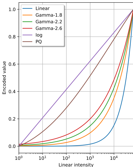
FIG. 7: TFs used in our experiments to map linear color values to the encoded values, suitable for CV methods.
