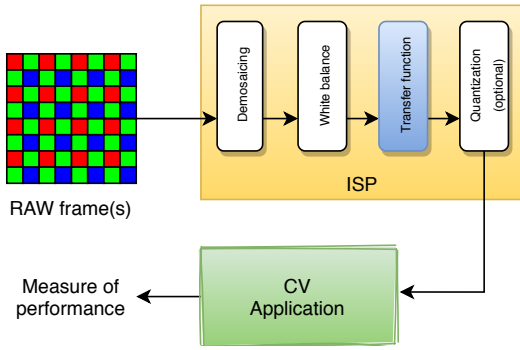
FIG. 6: The ISP pipeline used for evaluating the performance of CV methods. The intermediate frames are processed by a TF, followed by an optional quantization. This serves as an input to the CV application being tested.
