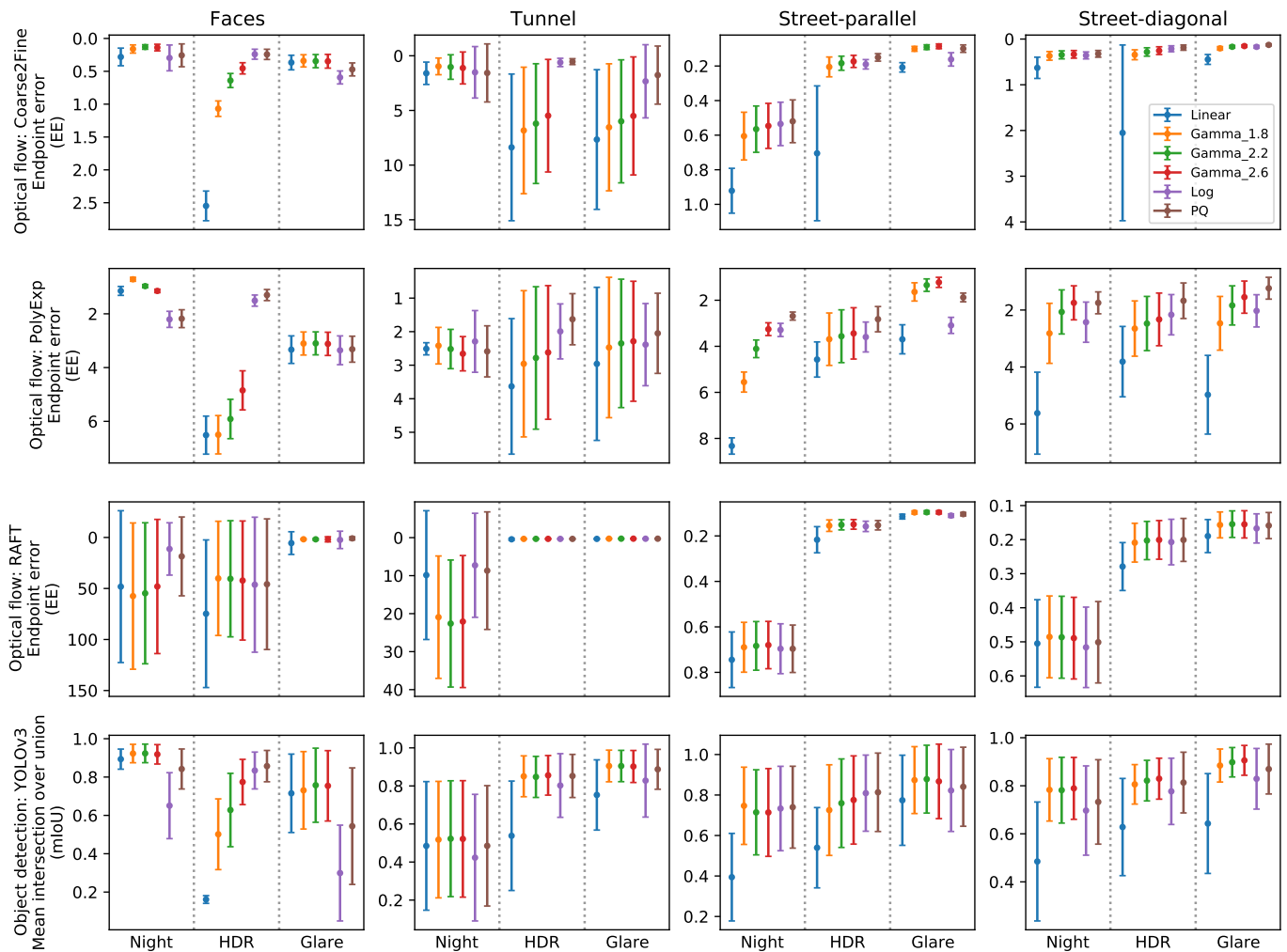
FIG. 8: The performance of optical flow (top three rows) and object detection (bottom row) for all four scenes (columns) and three adversarial illumination conditions (three sections in each plot). Dots represent the mean and the error bars represent the standard deviation for a sample of 100 frames. The y-axis is reversed for optical flow so that the points located higher on the plot correspond to the better performance.
