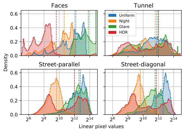
FIG. 4: Distribution of pixel values under different illumination conditions for all scenes in the dataset. Dashed vertical lines show the average pixel values under each illumination for each scene.
