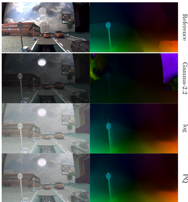
FIG. 9: Failure of gamma encoding for night condition of the Tunnel scene when the optical flow is estimated by RAFT. The purple region in optical flow visualization for gamma-2.2 indicates high velocity in the south direction, which is most likely caused by the dark region in that corner of the frame. The HDR TFs ( log and PQ ) can better handle this sequence. This is also the cause of the large error bars in some plots in Fig. 8
