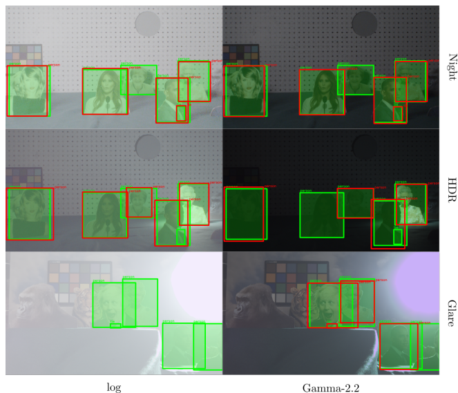
FIG. 10: Object detection using YOLOv3 for images captured under different illumination conditions (rows) and encoded with log (left column) and gamma (right column) TFs. The log function produces brighter images by devoting more bits to dark regions as indicated by the left plot in Fig 7. This leads to contrast reduction in bright regions posing problems to some object and face detectors for the Glare condition, but this is an effective strategy for other conditions.
