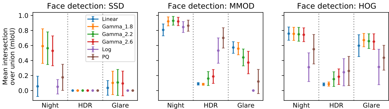
FIG. 11: The performance of face detection methods for all transfer functions and all illumination conditions. Dots represent sample mIoU, and error bars represent the sample standard deviation over 100 frames. When some transfer functions are used, some methods are unable to detect even a single face. For example, notice the zero entries for the HDR and glare illuminations with the log function for SSD and MMOD.
