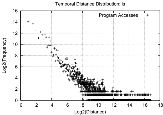
FIGURE 8. Temporal distance distribution of a trace for the Unix command ls , seems to exhibit approximately power-law behaviour.
