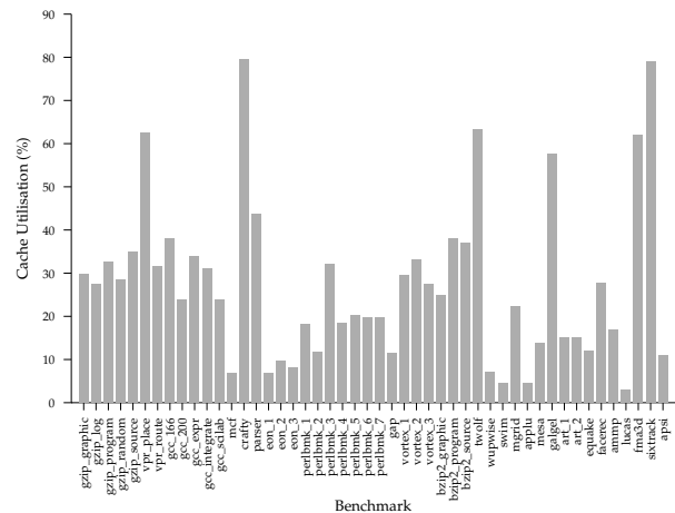
FIGURE 3. Level 2 cache utilisation (data kindly provided by James Srinivasan)
