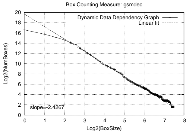
FIGURE 7. Box-counting measure of a GSM-decoder benchmark exhibits a power-law relationship between box-size and box-count. This indicates that the dynamic data-dependency graph for this algorithm exhibits fractal communication with a dimensionality, equal to its slope, of approximately 2.4.
