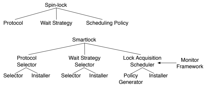
Figure 4: Smartlock Functional Design. A component to optimize each aspect of a lock.
