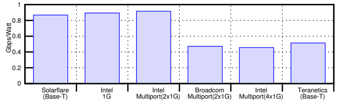
Fig. 4. 1 vs 10 Gbps - Performance-Per-Watt
