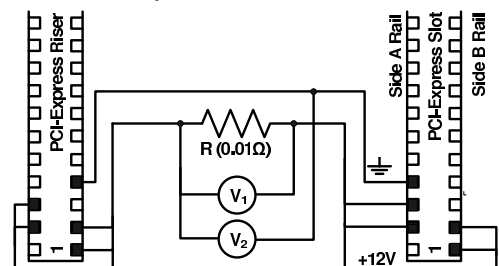
Fig. 1. 12v Power Measurement Apparatus
