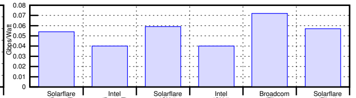
Fig. 3. 10 Gbps NICS – Server Performance Per Watt
